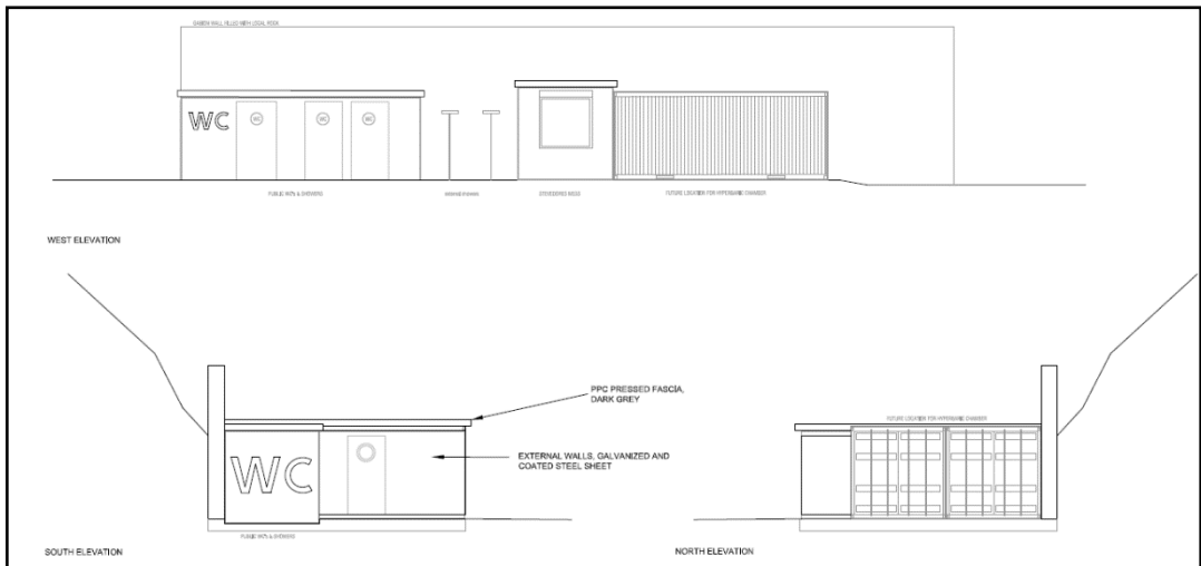
Diagram 5: Elevations of the Facilities
