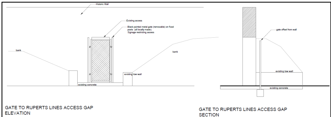
Diagram 6: Proposed Demountable Gate
