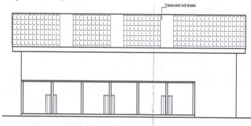
Diagram 5: Proposed East Elevations
