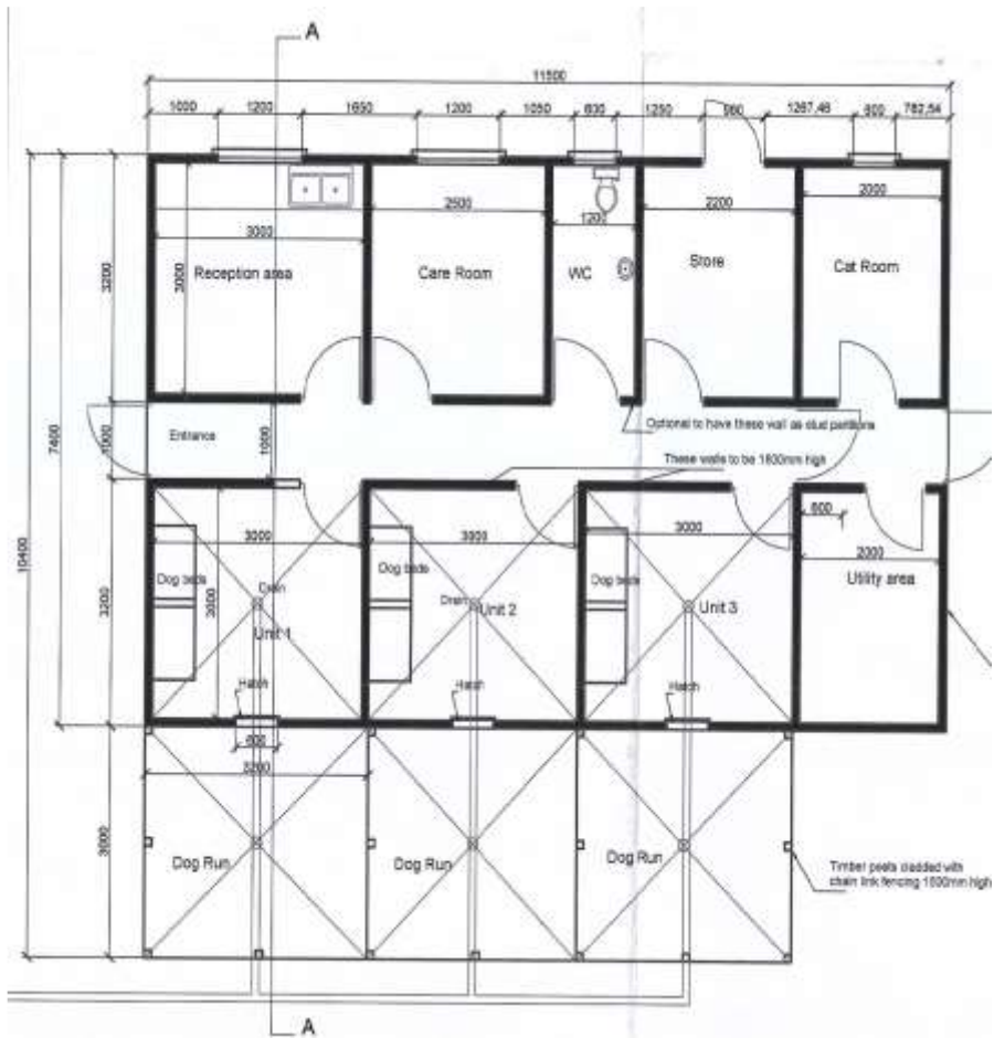
Diagram 3: Proposed Floor Layout
