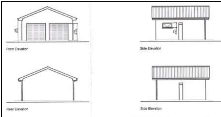
Diagram 4: Proposed Elevations
