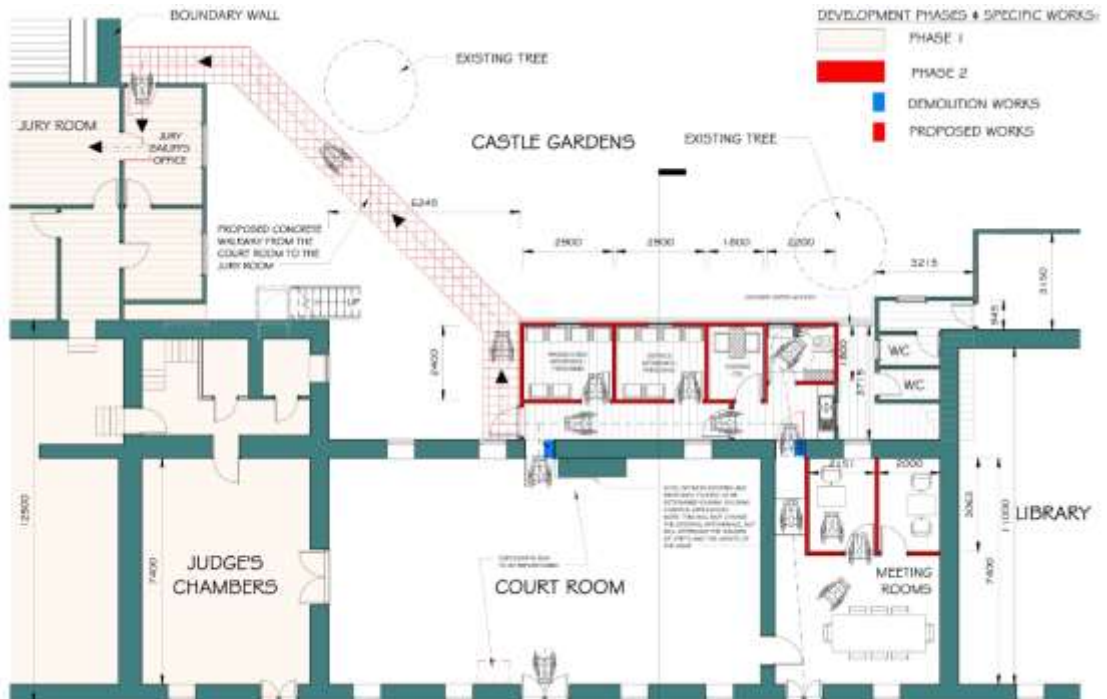
Diagram 5: Proposed Floor Layout
