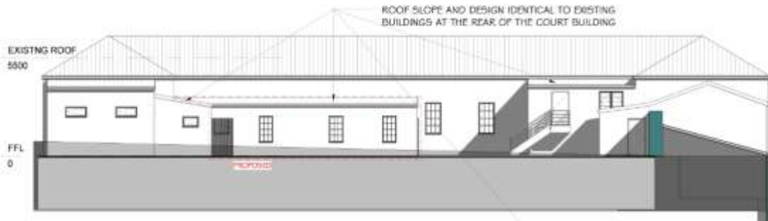
Diagram 3: Rear Elevation In Memorial Garden
