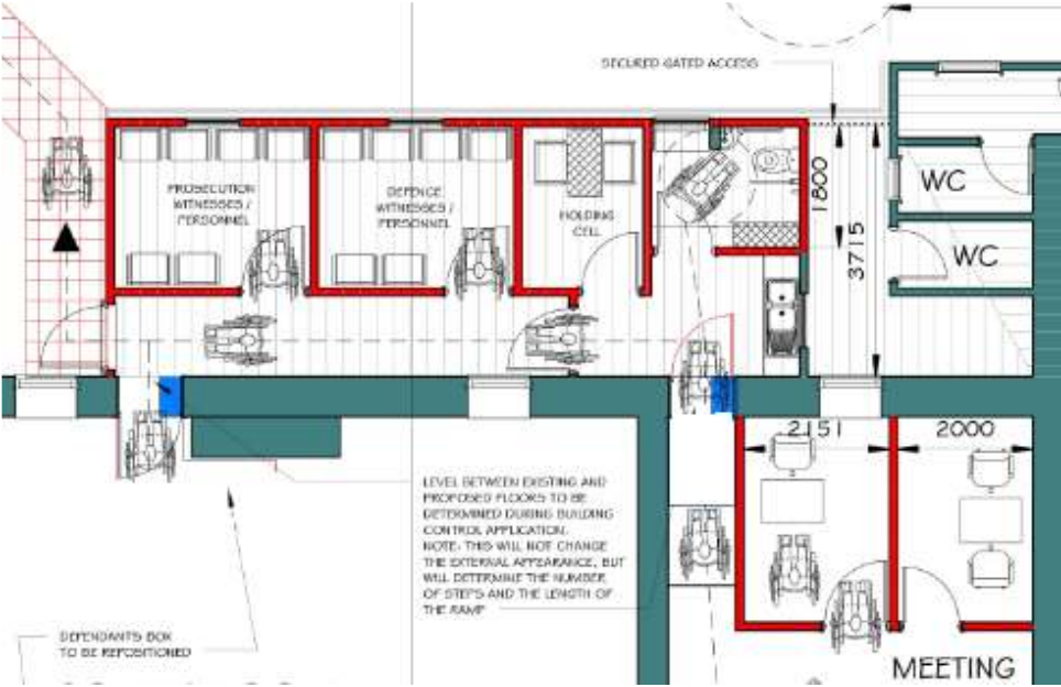
Diagram 6: Proposed Access Layout
