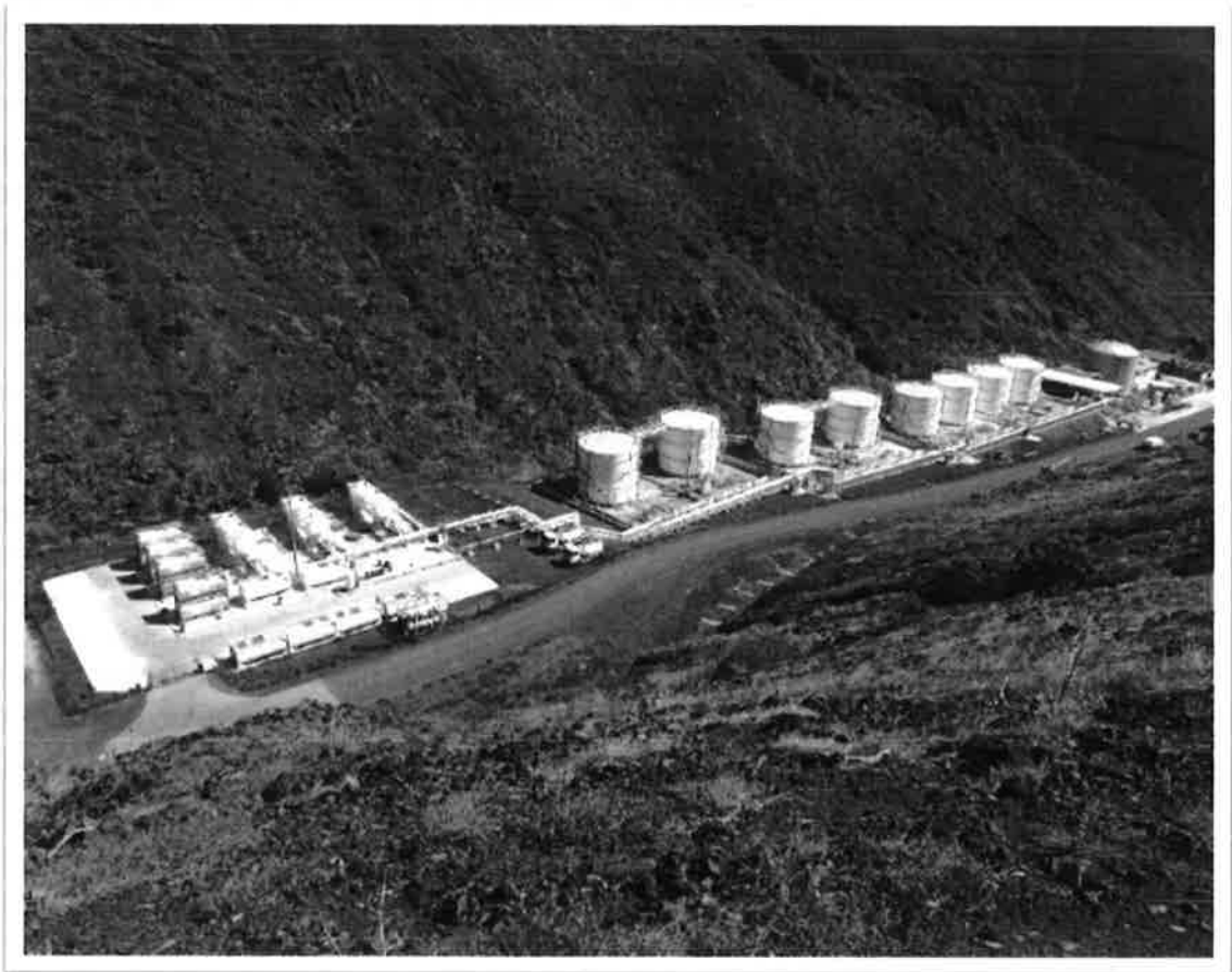
FIGURE 3. NEW BFI IN RUPERT'S VALLEY, DECEMBER 2018
