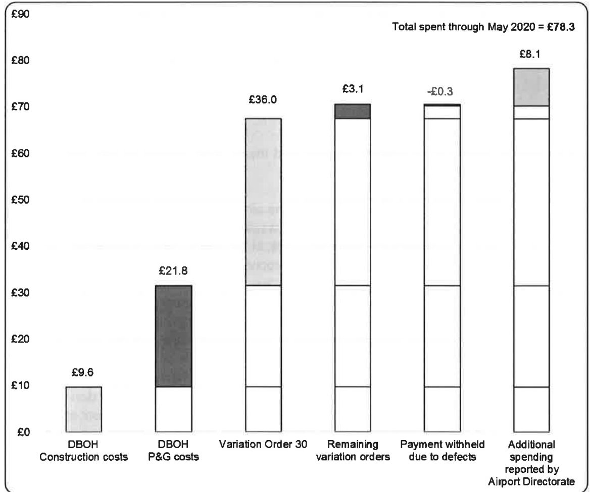
FIGURE 11. COMPOSITION OF TOTAL AMOUNT SPENT ON THE NEW FUEL SYSTEM THROUGH MAY 2020 (IN MILLIONS)
