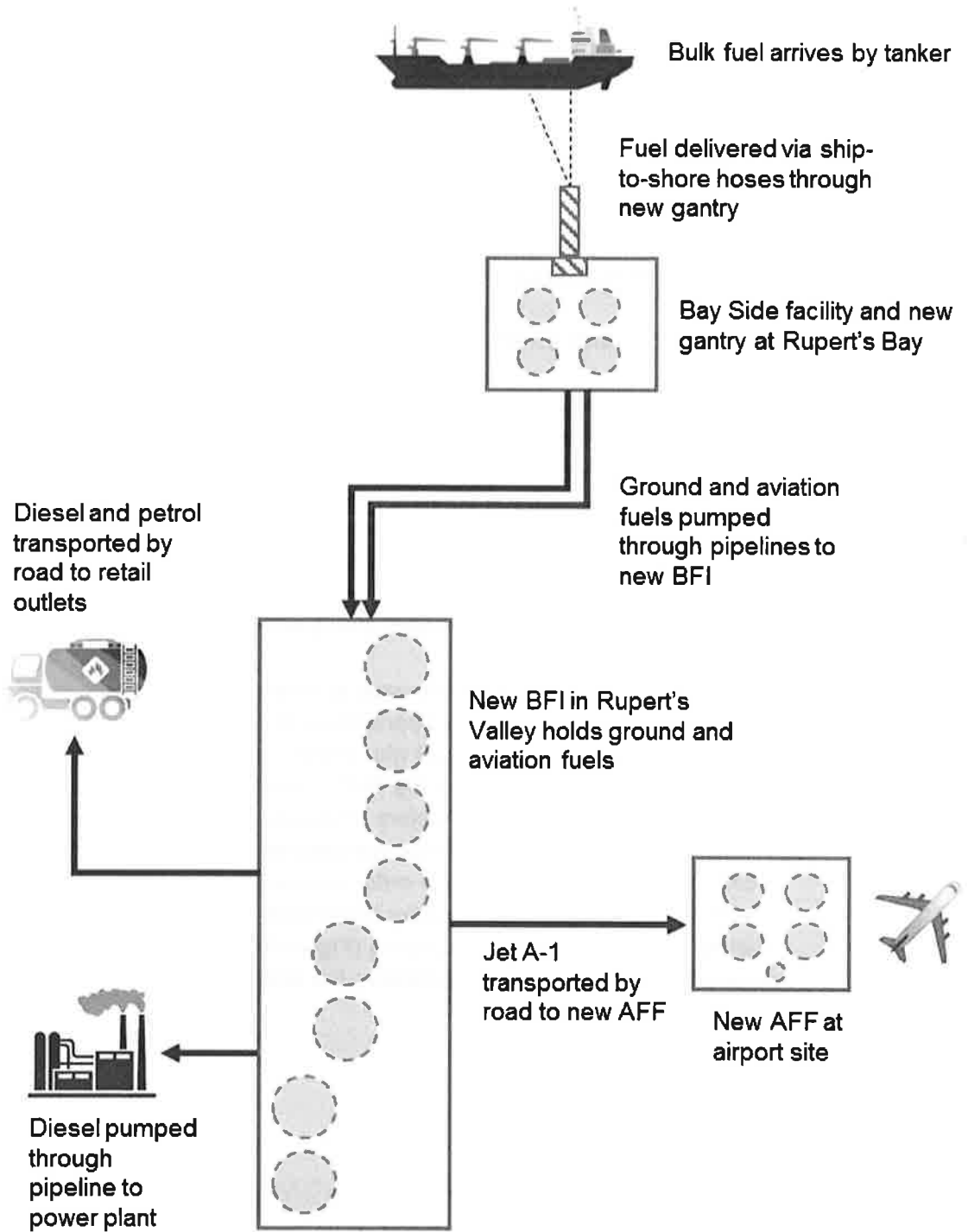
FIGURE 4. FUEL SYSTEM LAYOUT AS DESIGNED
