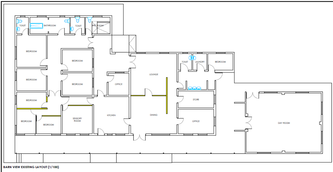
Diagram 2: Existing Floor Layout
