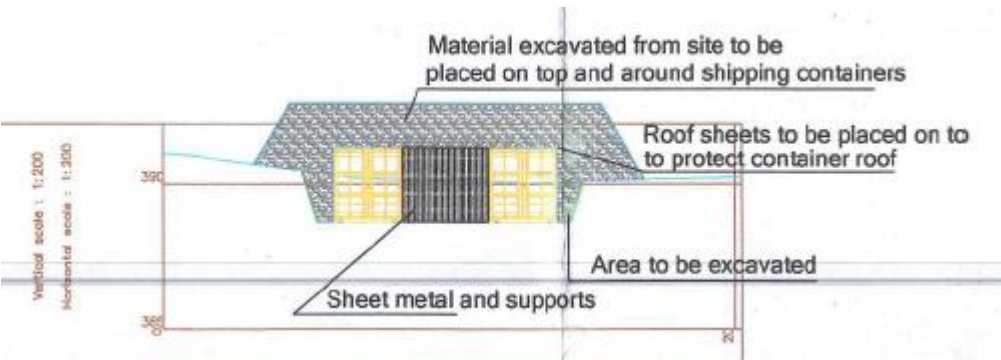
Diagram 4: Front Elevation
