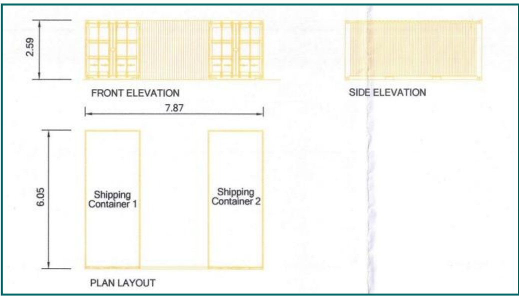
Diagram 6: Container Layout Plan
